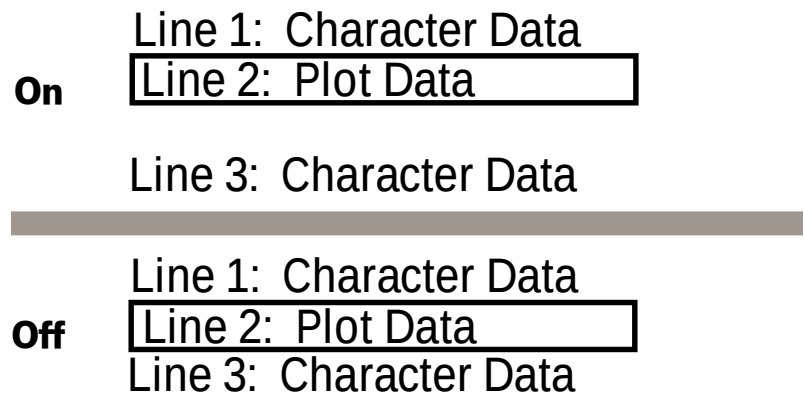
Figure 3 - 3. Modplot Example
